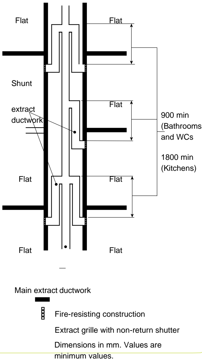
Figure 1 – Shunt duct arrangements
